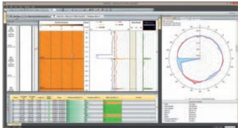
Casing Integrity Workspace (here with MFC data).
